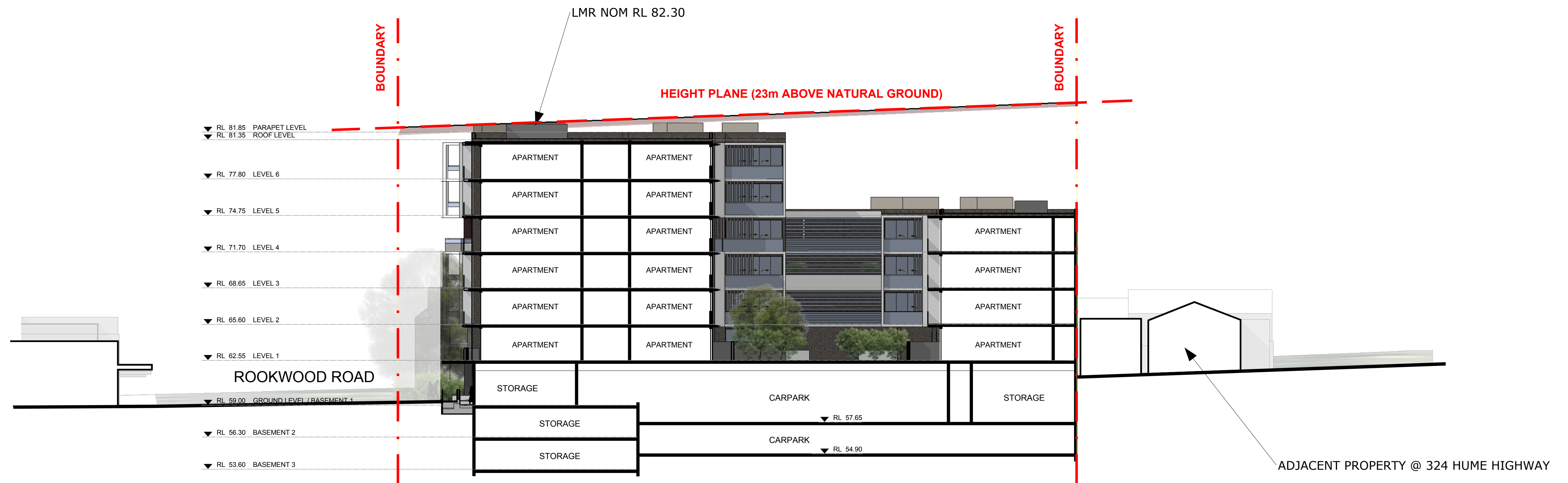
1 CROSS SECTION LOOKING NORTH
